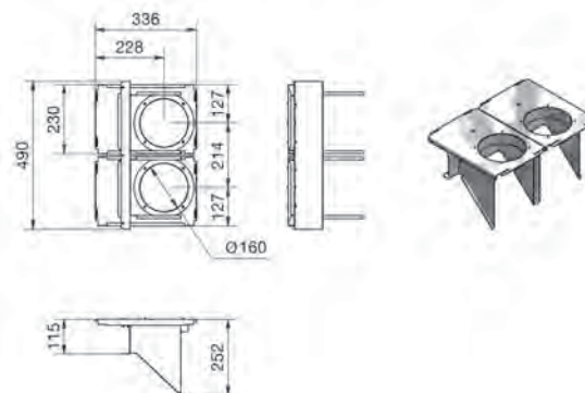
Zehnder ComfoAir 350
