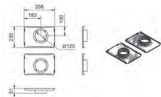
Zehnder ComfoAir 200
