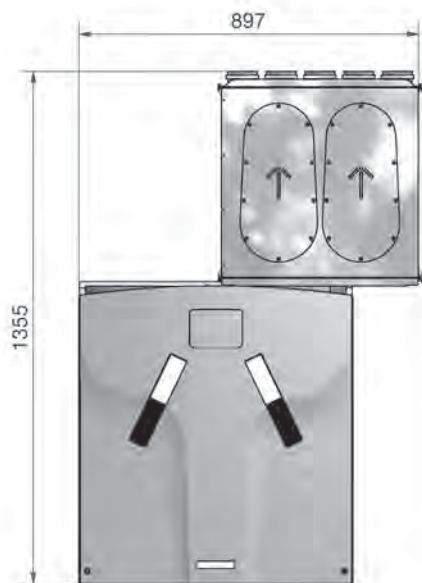
Zehnder ComfoAir 550
